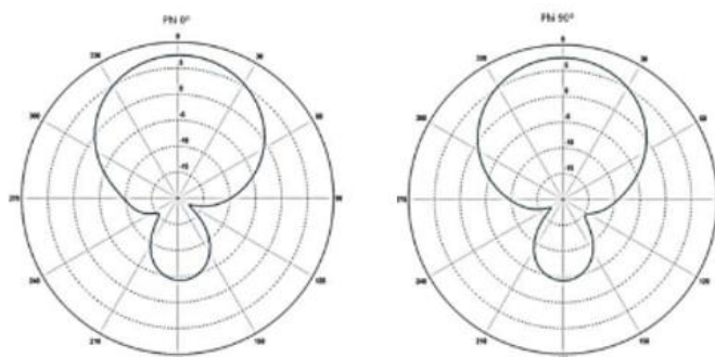
Figure 1: Radiation pattern of the internal antenna
