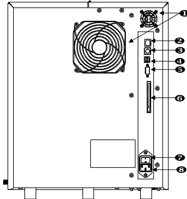
Figure 4. External Parts—Back
