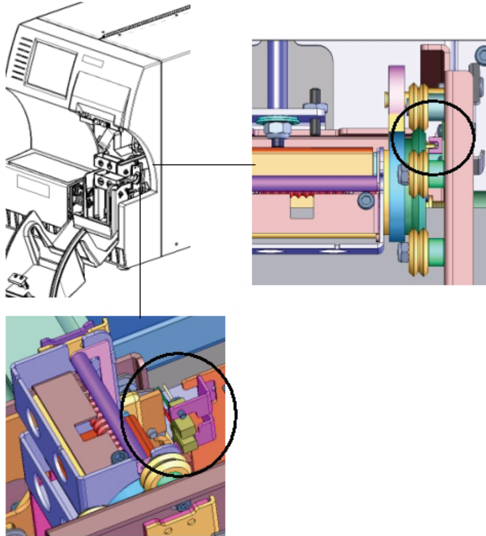
Figure 40. Wrapper and Shuttle Home Sensors
