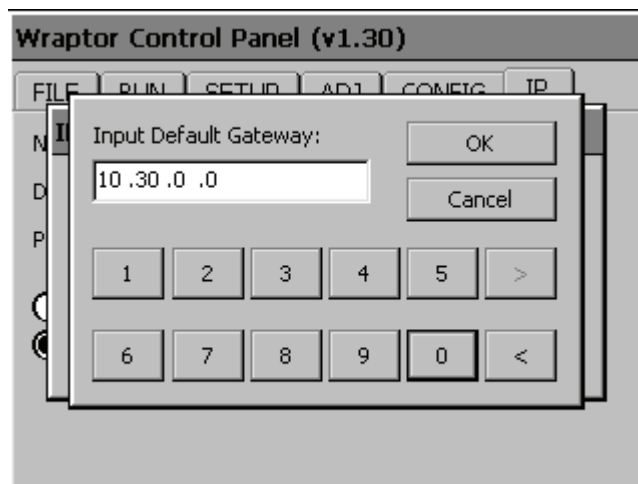
Figure 28. Default Gateway Entry
