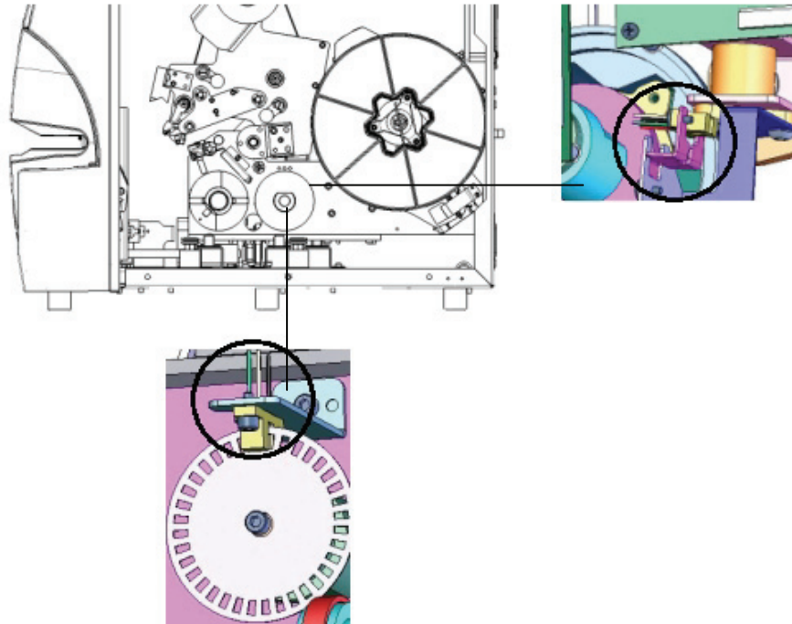
Figure 41. Tilt and Ribbon Out Sensors
