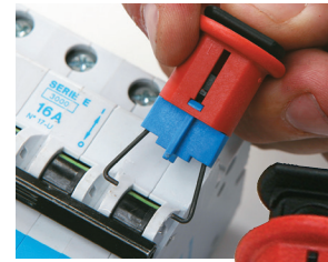
Pin-In Standard (PIS)
