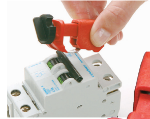
Tie-Bar Lockout (TBLO)
